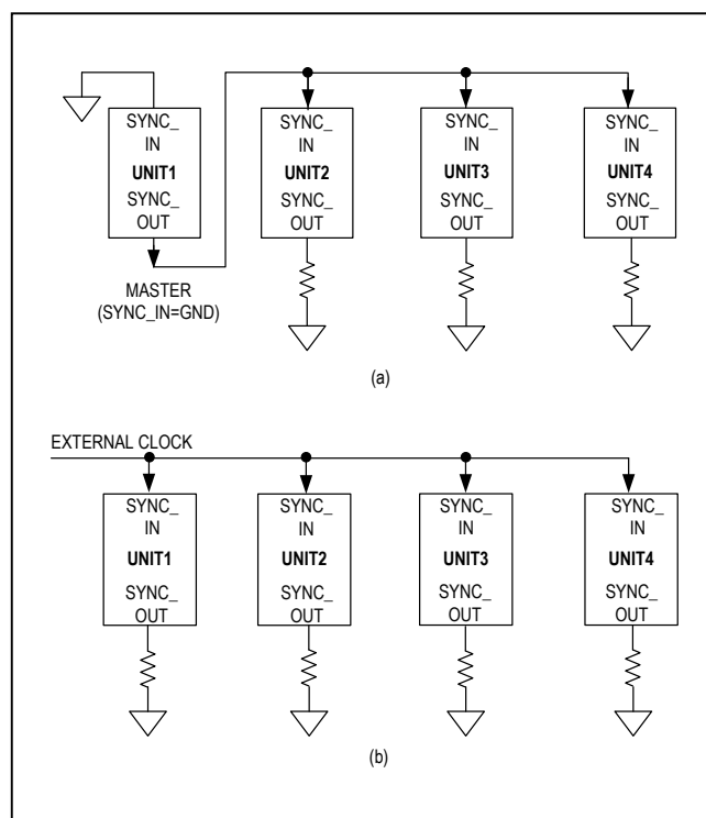
Figure 7. Synchronization Connection Diagram
