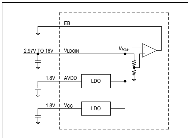
Figure 5. V_{I\_DOIN} with an External Supply Voltage
